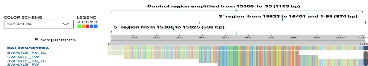
Figure S3. Multiple alignment and positioning of the four bidirectional sequences across the linearized circular mitochondrial genome of Balaenoptera physalus (GenBank accession MF409243.1), showing coverage of a 1109 bp consensus region spanning positions 15388 – 16401 and 1 - 95 of the mitochondrial control region.
