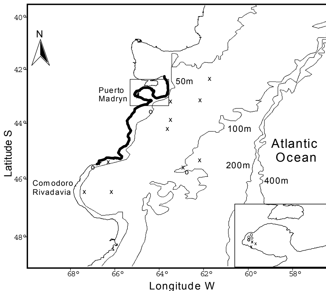
Figure 3. Location of Notorynchus cepedianus caught along the Patagonian shelf, indicating with circles those that consumed marine mammals and with crosses those that did not. Rookeries zones are shown with a thick line on the coast. At the bottom, a detail of Golfo Nuevo is shown.
